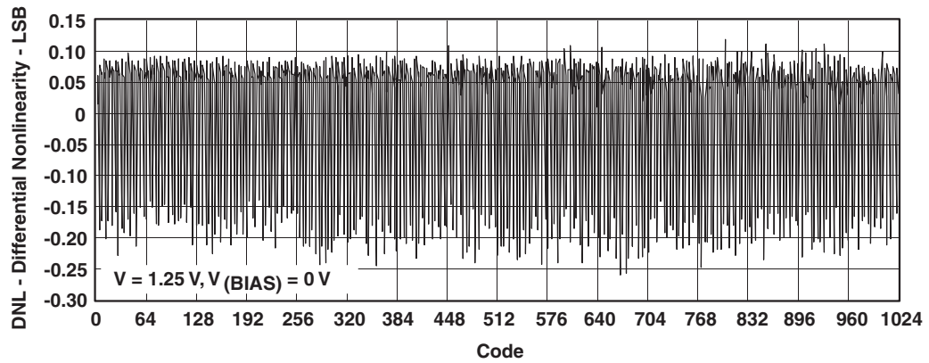
Figure 4-10. Differential Nonlinearity vs Code
