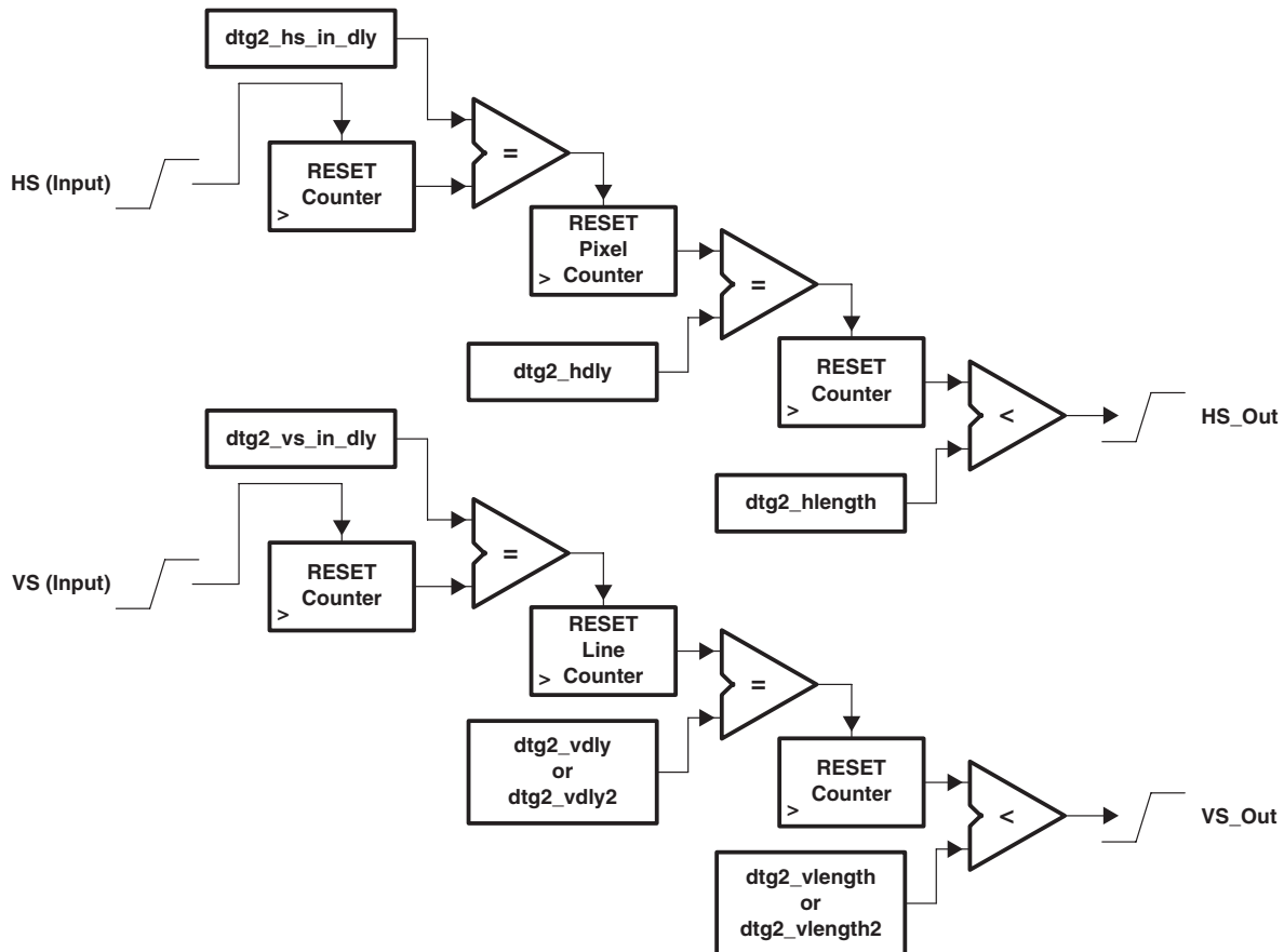
Figure 6-15. THS8200 DTG VS/HS Output Generation
