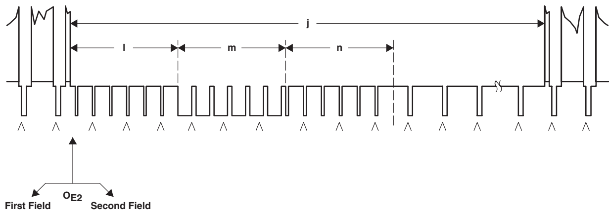
Figure 6-38. Field/Frame Synchronizing Signal Waveform (525I Format)
